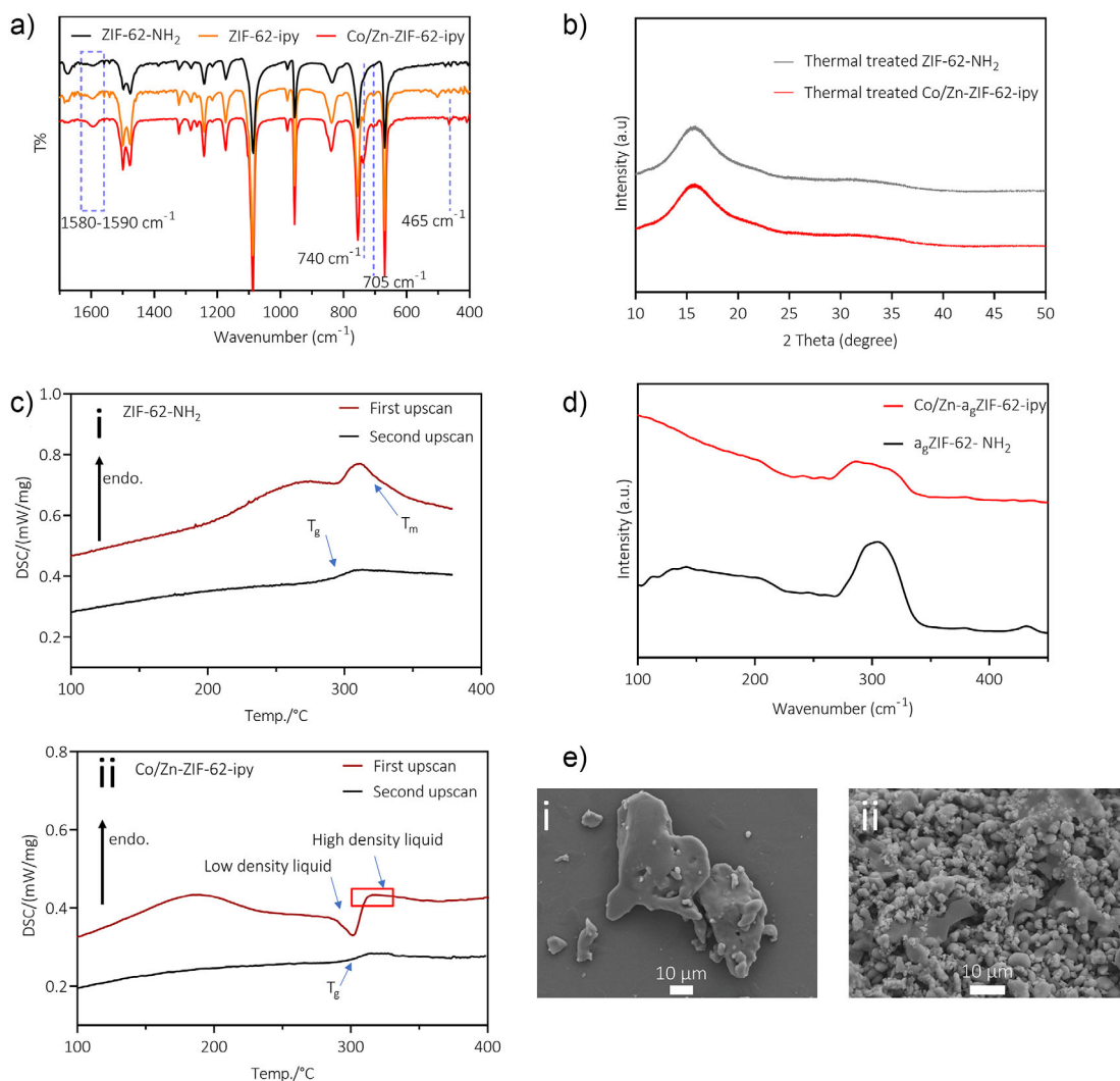
Figure 2. a) FTIR patterns of ZIF-62-NH 2 and its derivative ZIF-62-ipy and Co/Zn-ZIF-62-ipy. b) PXRD patterns of a g ZIF-62-NH 2 and Co/Zn-a g ZIF-62-ipy. c) DSC curves of (i) ZIF-62-NH 2 and (ii) Co/Zn-ZIF-62-ipy, the first upscan recorded the LLT and the second upscan exhibited T g . d) THz/Far-IR spectrums for a g ZIF-62-NH 2 and Co/Zn-a g ZIF-62-ipy. e) SEM image of (i) a g ZIF-62-NH 2 and (ii) Co/Zn-a g ZIF-62-ipy.
