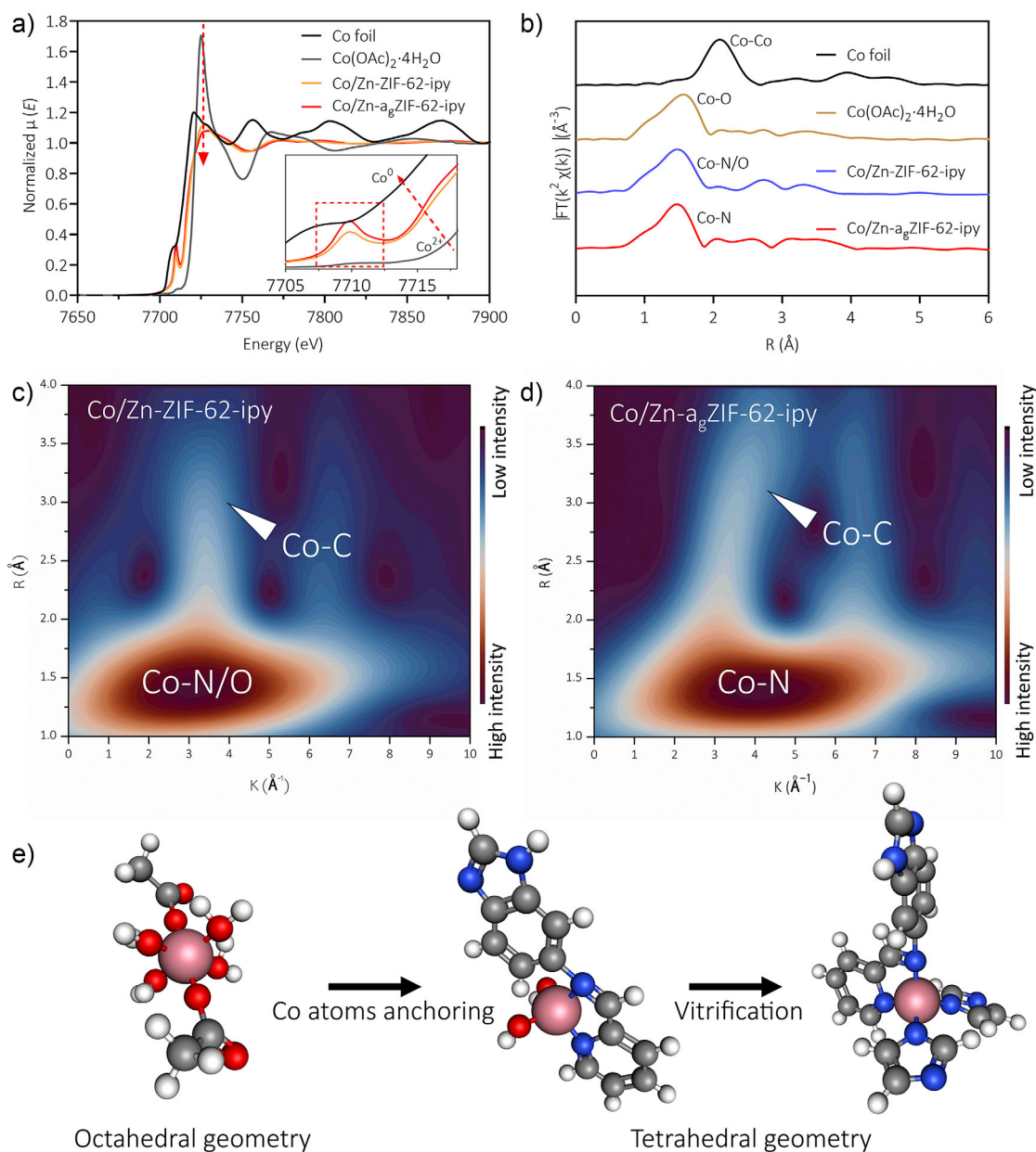
Figure 3. a) Co K-edge XANES spectra. The inset is an enlargement of the Co pre-edge peak. b) EXAFS for Co foil, Co(OAc) 2 ·4H 2 O, Co/Zn-ZIF-62-ipy, and Co/Zn-a g ZIF-62-ipy, respectively. c) WT plot for Co from Co/Zn-ZIF-62-ipy. d) WT plot for Co from Co/Zn-a g ZIF-62-ipy. e) Cobalt local coordination environment changed upon anchoring and vitrification. Co, O, C, H, and N atoms are represented as pink, red, grey, white, and blue spheres, respectively.
